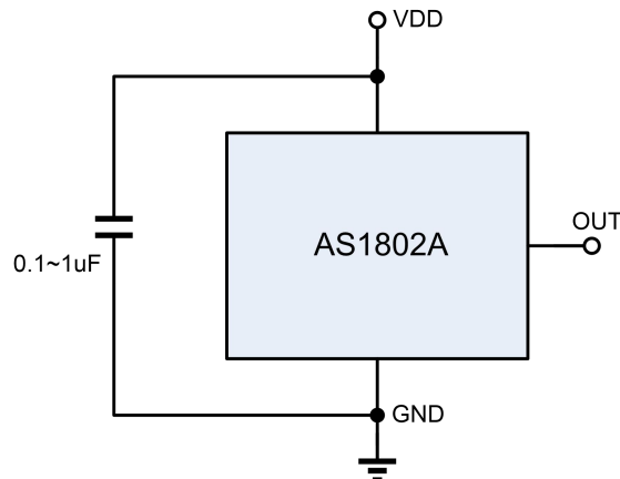
Figure 1, Typical Application Circuit of AS1802A
