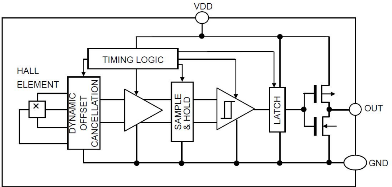
Figure 2, Block Diagram of AS1802A
