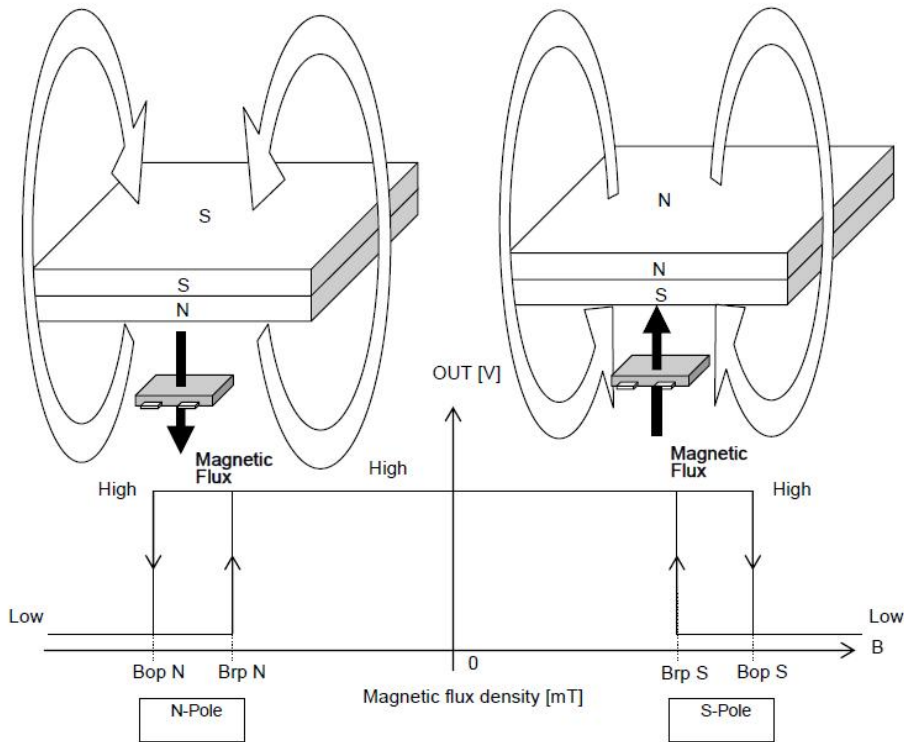
Fig 3, Magnetic Operation Characteristic of AS1802A
